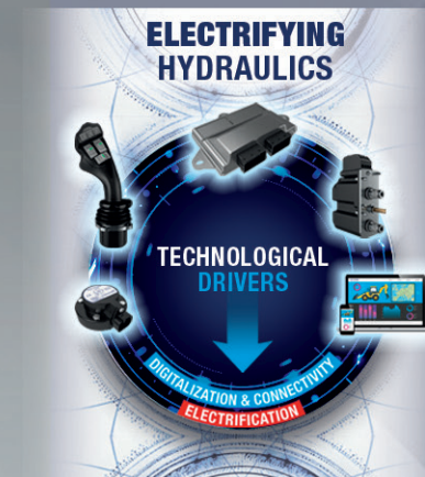
Digitalization
